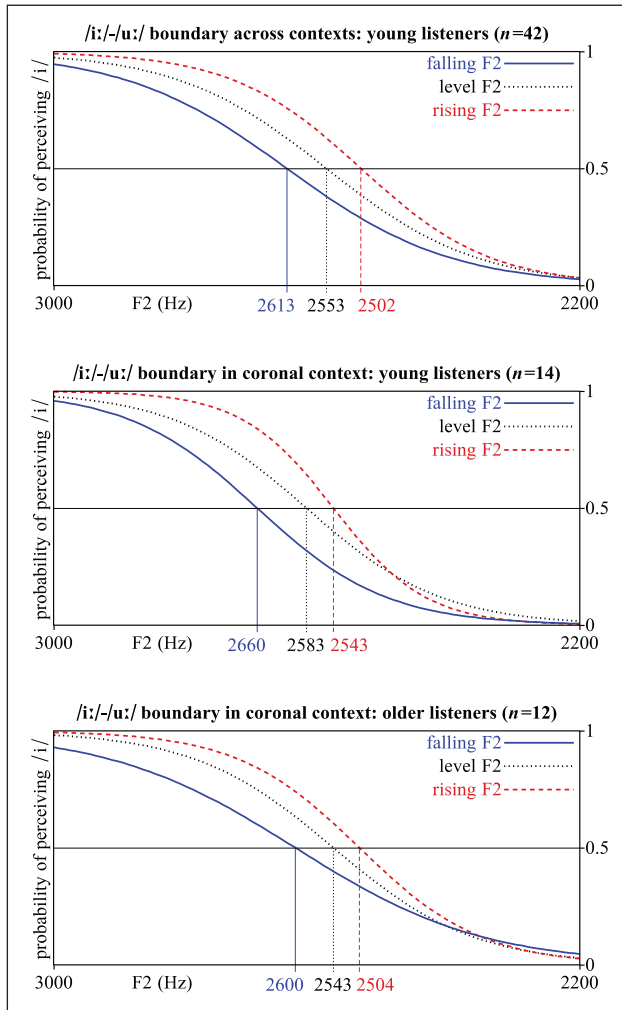
Figure 5. Experiment 2: perceptual /i:/-/u:/ boundaries on the F2 dimension, averaged across n listeners in each group. The top graph shows results for the 42 young listeners. The middle graph shows the subgroup of 14 young listeners who were directly compared to the 12 older listeners (shown in the bottom graph). Note that in order to zoom in on the boundary locations, the graphs show an F2 range between 2200 and 3000 Hz, however, the stimulus continuum in the experiment ranged from 1800 to 3200 Hz.
