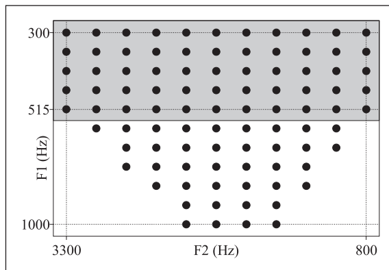
Figure 6. Experiment 3: the sampling of the F1–F2 stimulus space. The 55 F1–F2 pairs in the upper gray region were synthesized with two F3 values, two durations, and three trajectory types. The remaining F1–F2 pairs from the lower region were synthesized with one F3 value, one duration, and one trajectory type (level).
