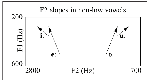
Figure 1. A visualization of the trend in formant slope directions for non-low vowels observed in several languages (see studies discussed in text): the F1 slope tends to be falling, whereas the F2 slope tends to be rising for the front vowels and falling for the back ones. This effect is seen for vowels produced in isolation as well as for vowels produced in various consonantal contexts (when consonant-specific formant transitions are removed, that is, in the central 50% portion of vowels). Note that the exact F1 and F2 locations of the arrows are illustrative and depict the general tendencies observed across languages.
