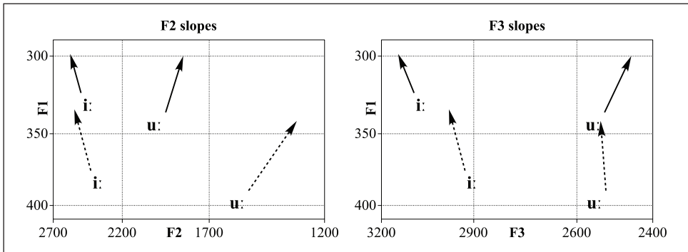
Figure 3. Formant values measured at 25% (start points of the arrows) and 75% (end points of the arrows) of the vowels' total duration, averaged across the four speakers per age group. Solid lines = younger speakers, dashed lines = older speakers. The average formant slopes were: 0.6-ERB fall for F1, 0.33-ERB rise for F2 of /i:/, 0.85-ERB fall for F2 of /u:/, 0.14-ERB rise for F3 of /i:/, and 0.09-ERB fall for F3 of /u:/. In order to show the magnitude of formant changes along a psychoacoustically plausible scale, the formant changes are given in ERB, and so is the scaling of the axes in the figure.
