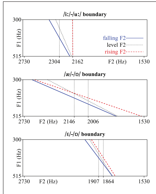
Figure 8. Experiment 3: perceptual front–back phoneme boundaries in the two-dimensional F1–F2 space, split into separate graphs for each vowel contrast. Boundaries are shown for every F2 slope type separately, coded by color and line-type (blue solid line = boundary for falling F2 slope; black dotted line = boundary for level F2; red dashed line = boundary for rising F2 slope). The boundaries were obtained from the logistic regression coefficients \beta_1 and \beta_2 for the regression factors midpoint F1 and midpoint F2, using the formula x = -\frac{\beta_0 + \beta_1 y}{\beta_2} , where x represents midpoint F1 and y represents midpoint F2 values.
