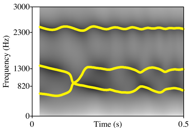
Figure 3: Long-window LPC spectrogram.
