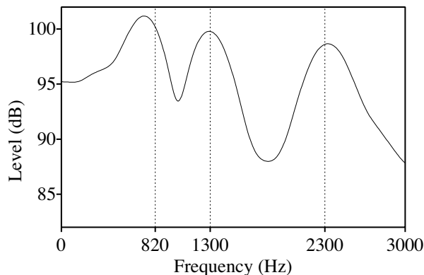
Figure 7: Truncated-filter spectrum.
