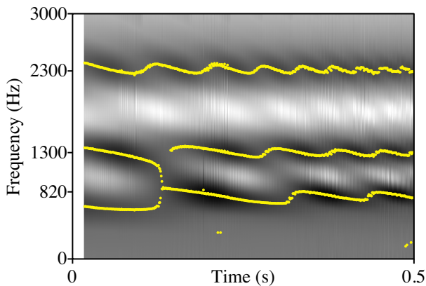
Figure 4: Interpolated pitch-related Fourier spectrogram
